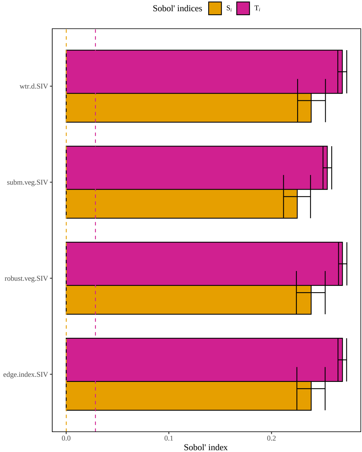
Figure 5. Results of a sensitivity analysis for the yellowheadedblackbird model based on a geometric mean structure. Dashed lines represent baseline numerical approximation error for S_i and T_i ( i.e. , dummy variables).
