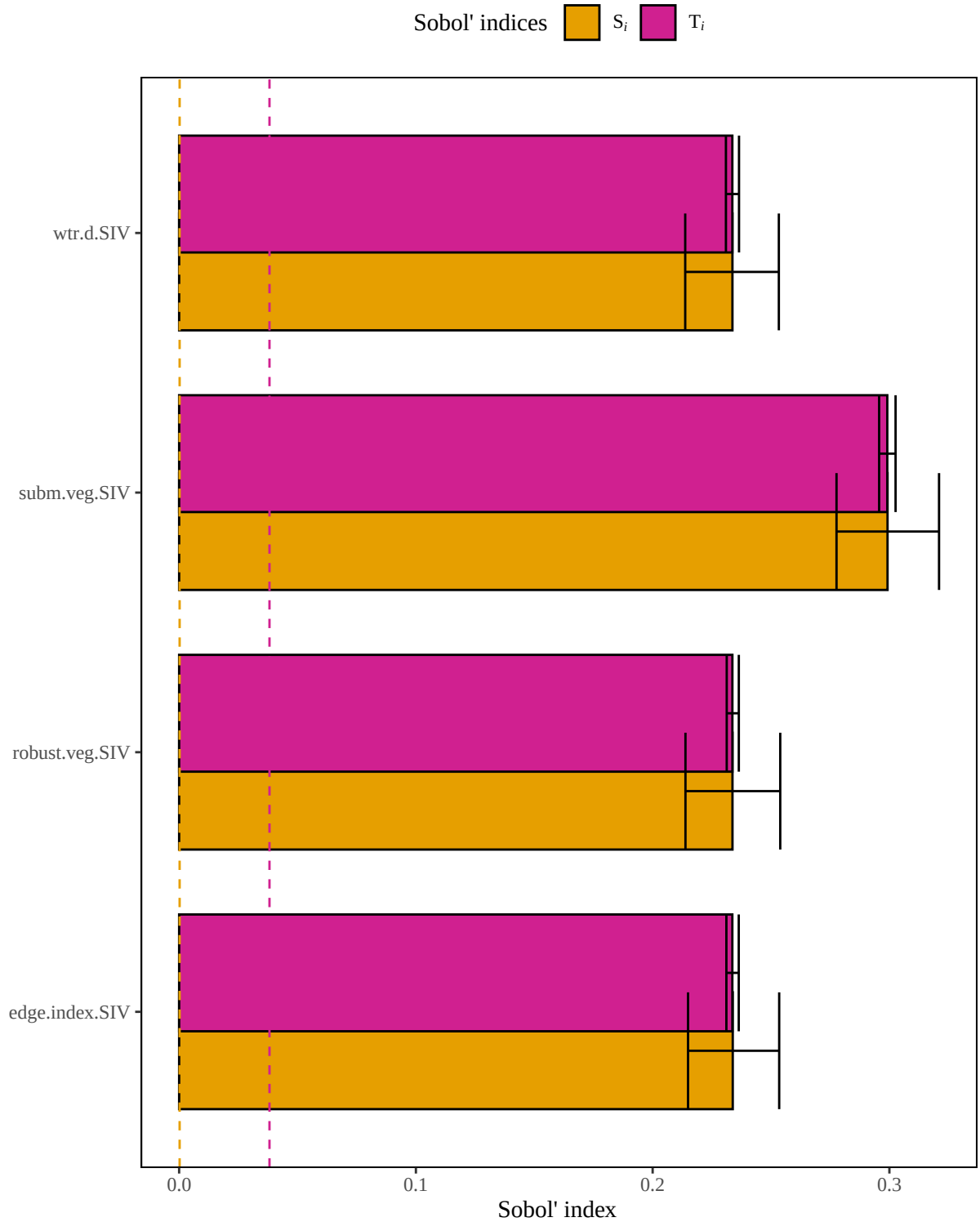
Figure 4. Results of a sensitivity analysis for the yellowheadedblackbird model based on an arithmetic mean structure. Dashed lines represent baseline numerical approximation error for S_i and T_i ( i.e. , dummy variables).
